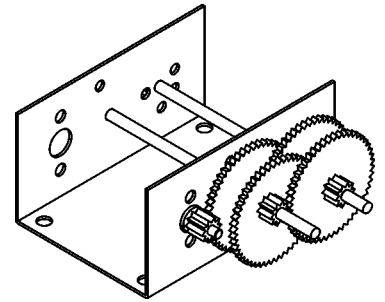
The MULTI-RATIO GEARBOX
