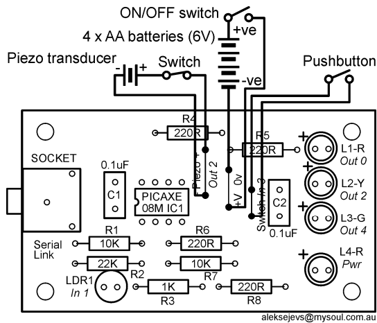
WIRING DIAGRAM
