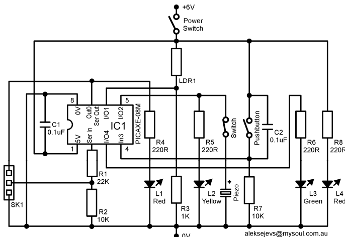
CIRCUIT DIAGRAM
