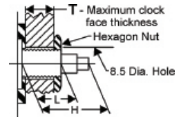
USING THE SUPPLIED HEXAGON NUT
