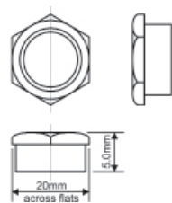
EXTENSION NUT Code: ENUT5 Price ea.: $0.48
