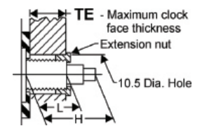
USE AN EXTENSION NUT for 2.0mm thicker material
